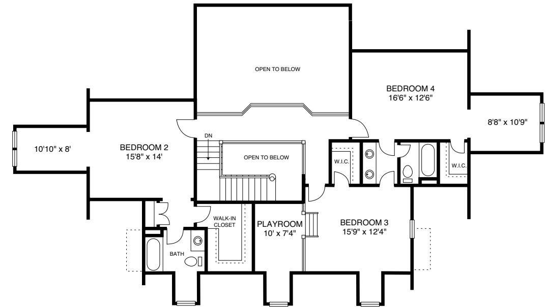
Second Floor
