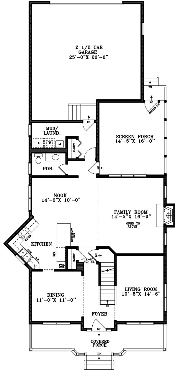
FIRST FLOOR PLAN 1,200 SQ. FT.
