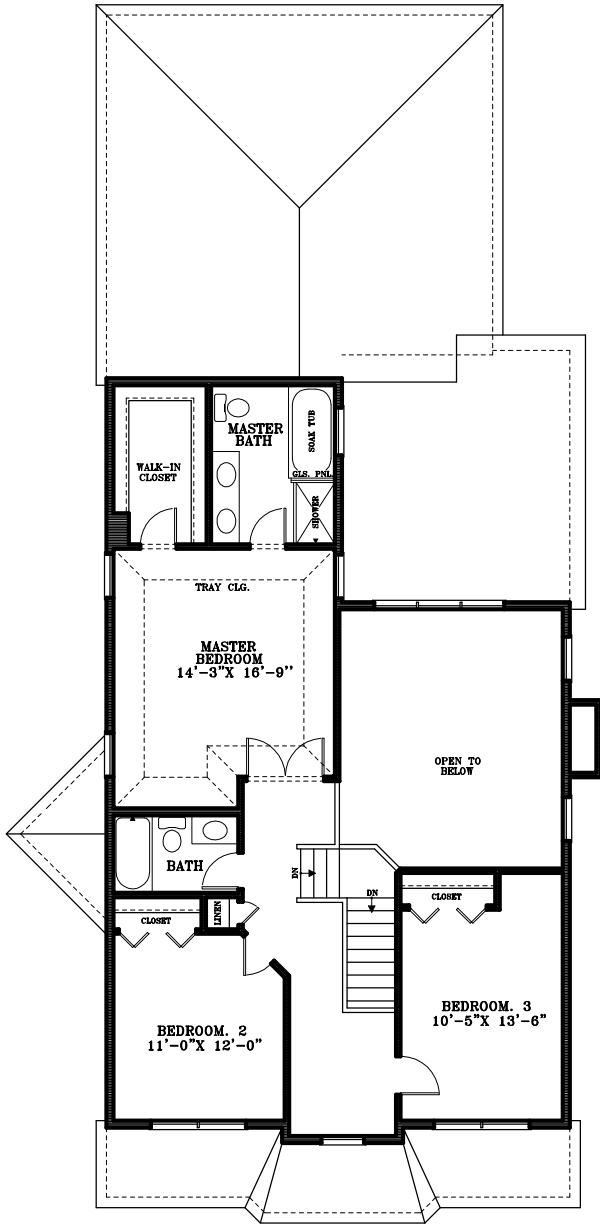
SECOND FLOOR PLAN 997 SQ. FT.
