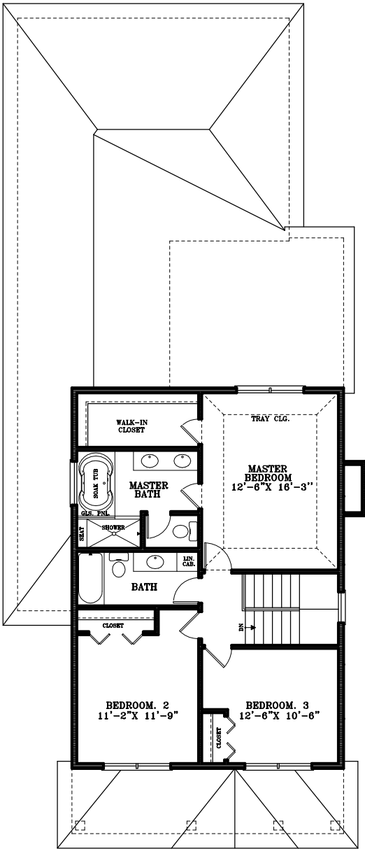
SECOND FLOOR PLAN 875 SQ. FT.
