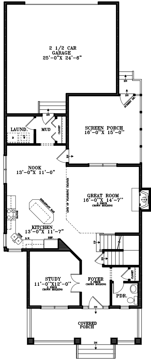
FIRST FLOOR PLAN 1,037 SQ. FT.
