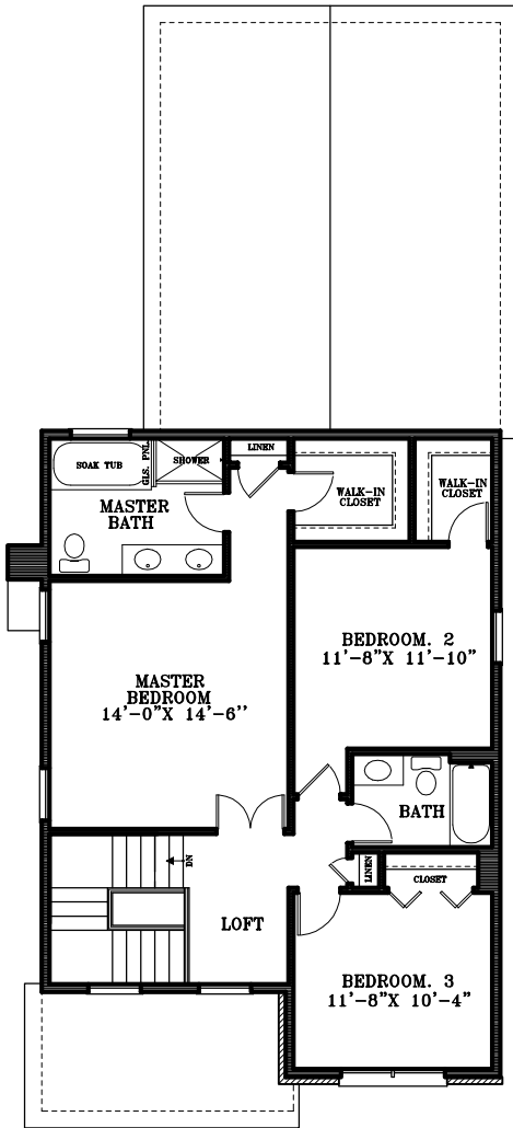
SECOND FLOOR PLAN 962 SQ. FT.
