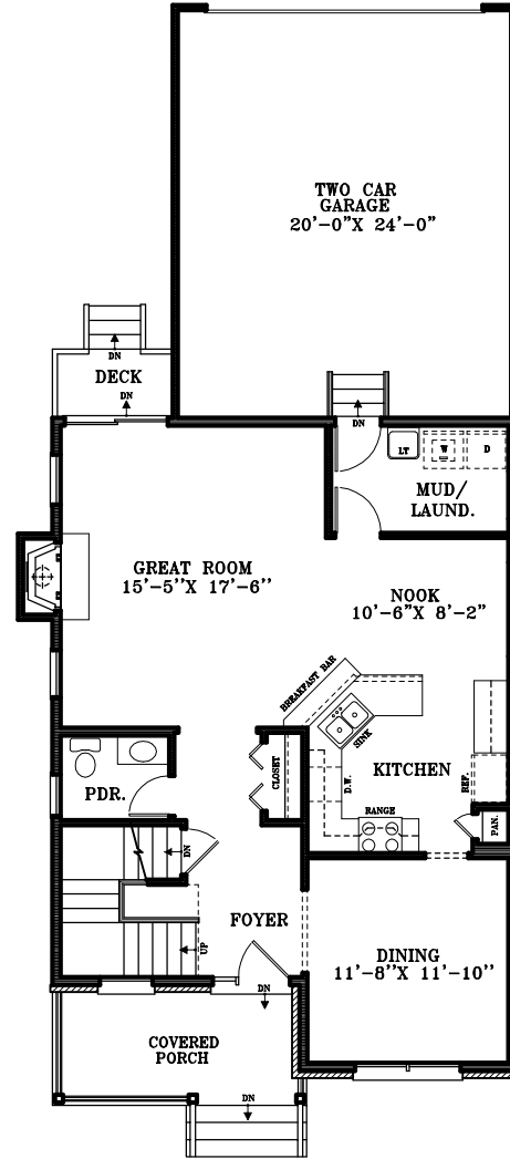
FIRST FLOOR PLAN 967 SQ. FT.
