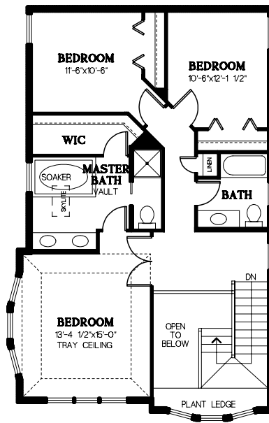
SECOND FLOOR PLAN 934 SQUARE FEET
